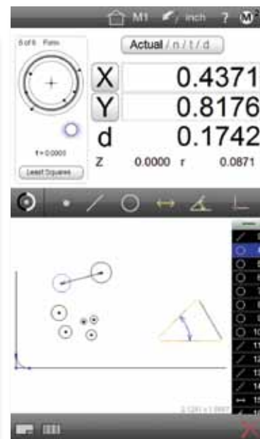
Circle geometry
